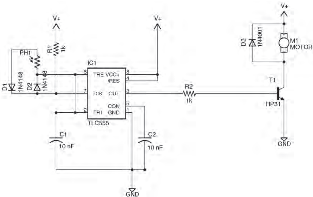
Figure 4: Circuit Diagram for TatlinTower Headdress, 2012 (© John Richards).
